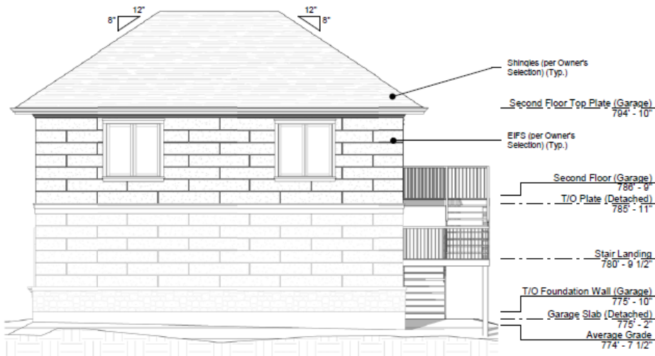
5 Detached Garage West Elevation
