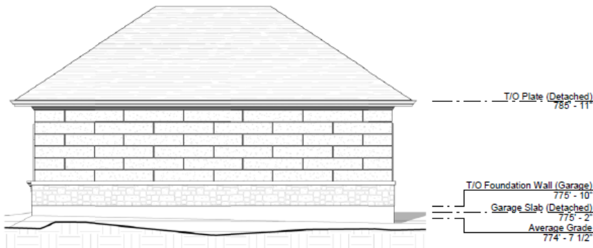
6 Detached Garage West Elevation - Existing
