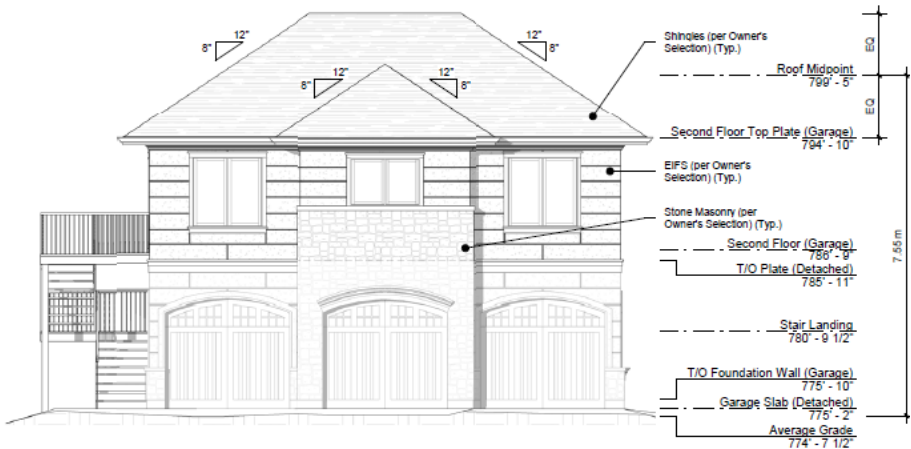
3 Detached Garage East Elevation
