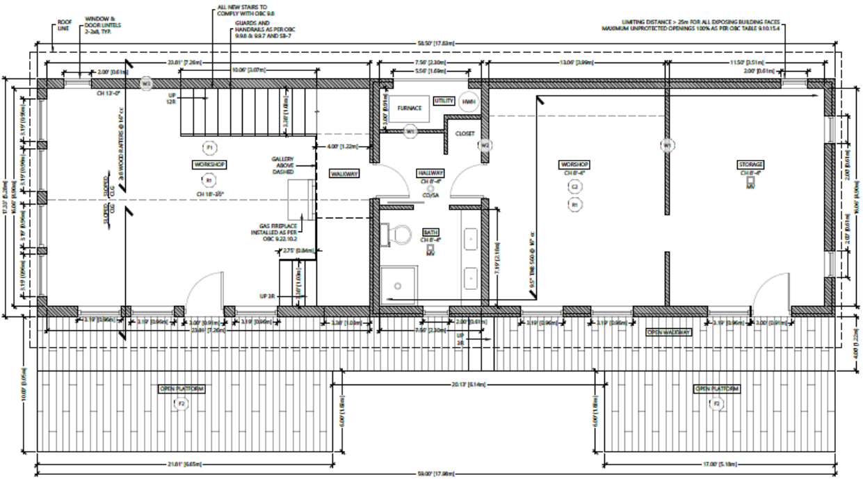
Floor Plan (Main Floor):
