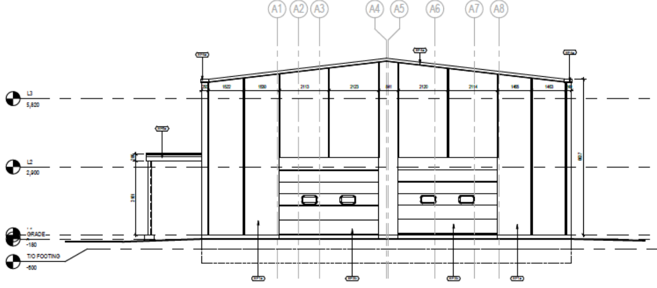
1 EAST ELEVATION 1 : 75
