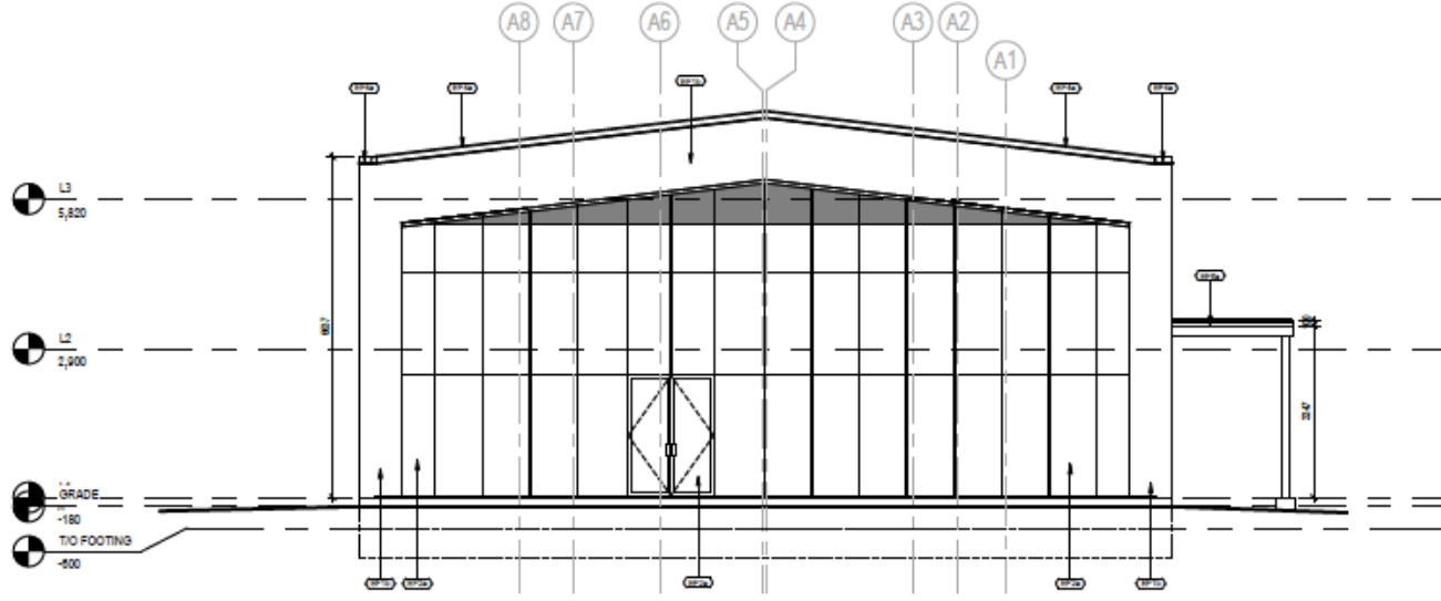
2 WEST ELEVATION 1 : 75
