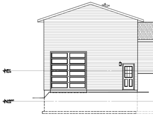
PART EAST ELEVATION
