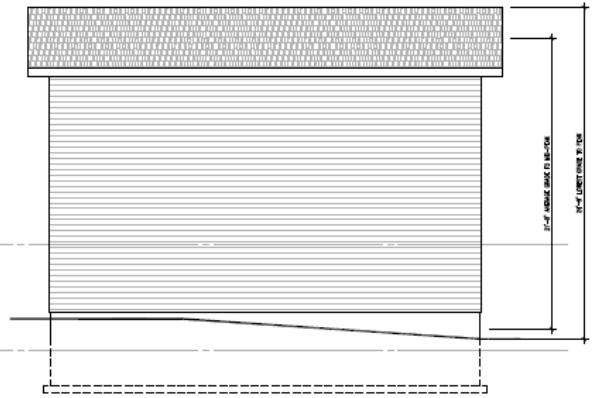
PART SOUTH ELEVATION
