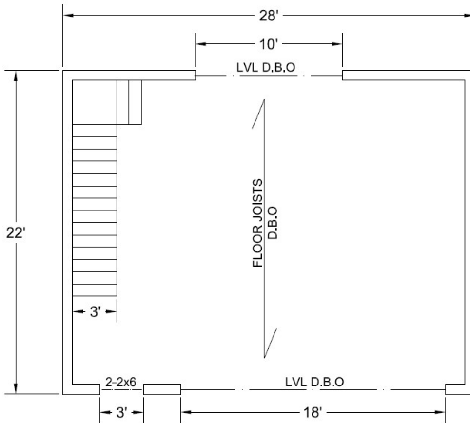
MAIN FLOOR PLAN 1/4" = 1'-0"
