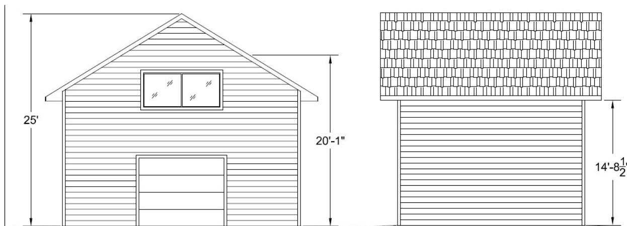
REAR ELEVATION 3/16" = 1'-0"
