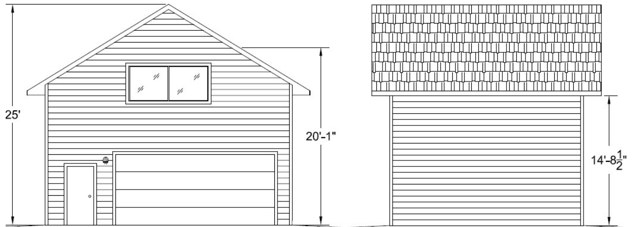
FRONT ELEVATION 3/16" = 1'-0"
