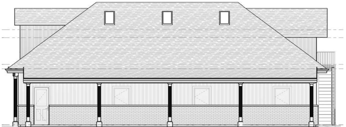
4 NORTH ELEVATION A2 1/4" = 1'-0"
