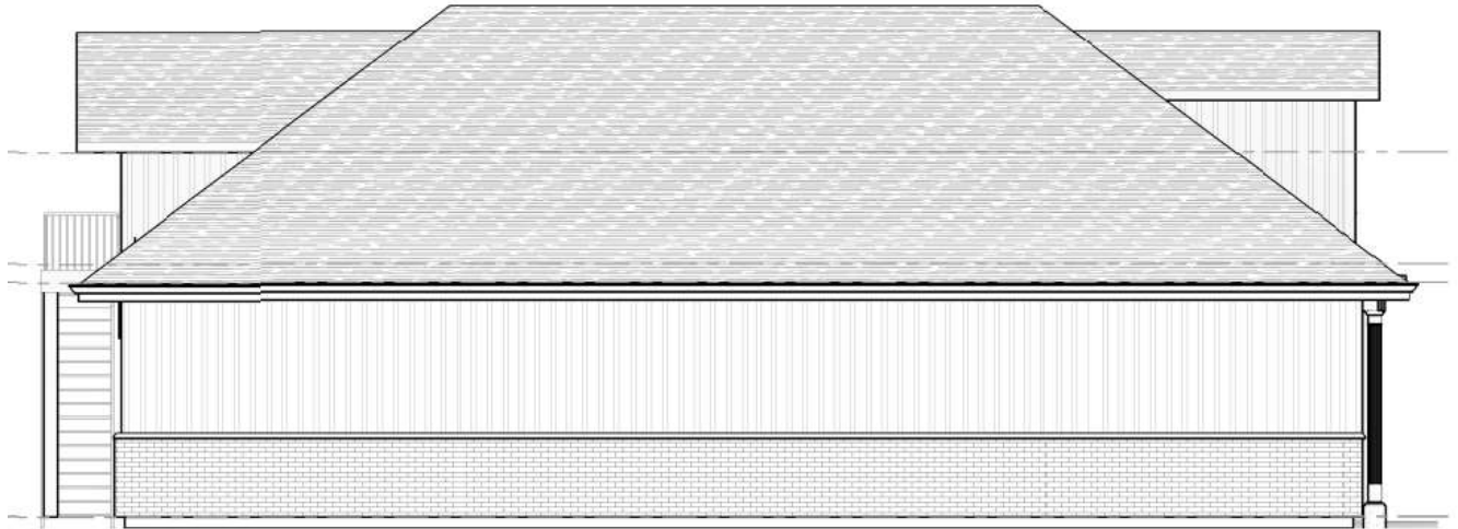
2 SOUTH ELEVATION A3 1/4" = 1'-0"
