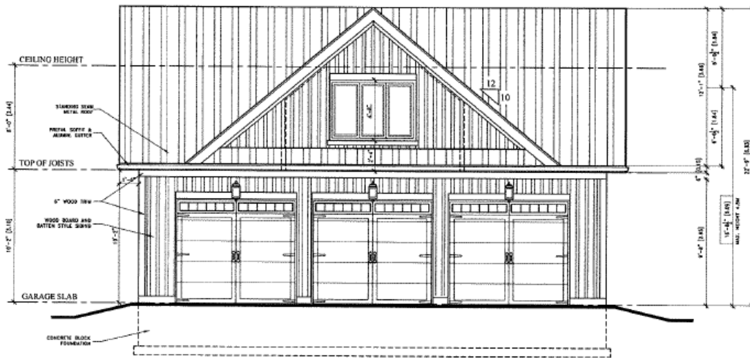
SOUTH ELEVATION
