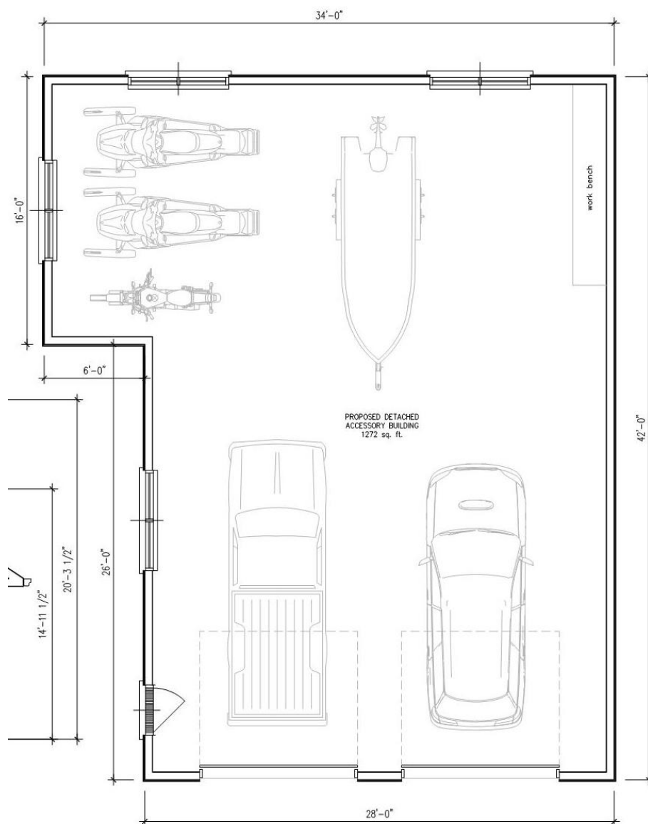
FLOOR PLAN
