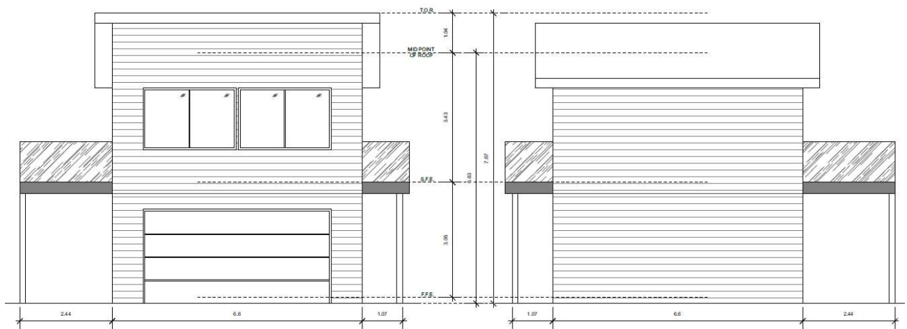
Front and Rear Elevations
