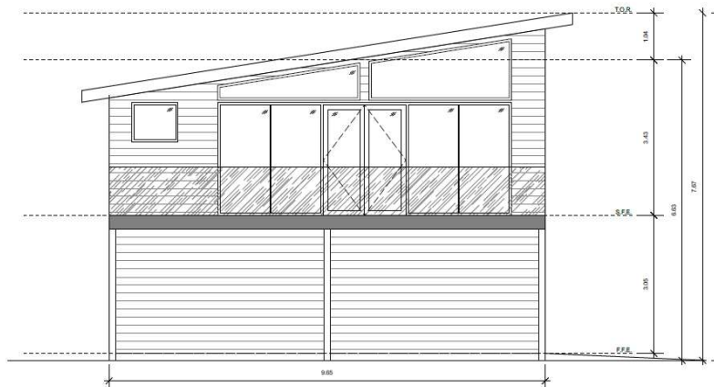
East Elevation
