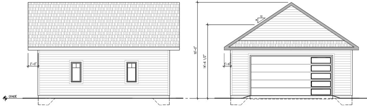
NORTH ELEVATION
