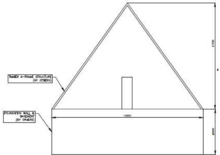
4 B6 *PROPOSED GUEST SERVICES BUILDING N.T.S. ELEVATION
