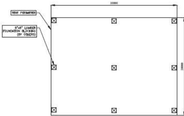
1 B6 *PROPOSED MULTI-PURPOSE TENT N.T.S. PLAN
