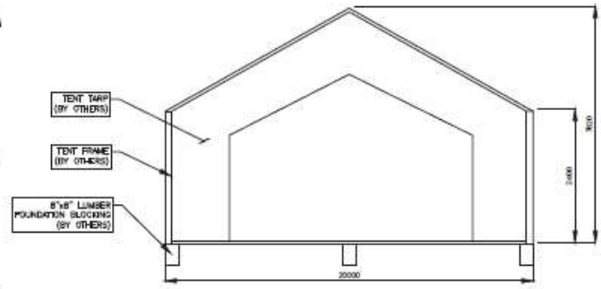
2 B6 *PROPOSED MULTI-PURPOSE TENT N.T.S. ELEVATION
