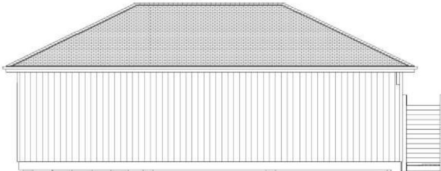
EXTERIOR ELEVATION SCALE: 3/16" = 1' - 0"
